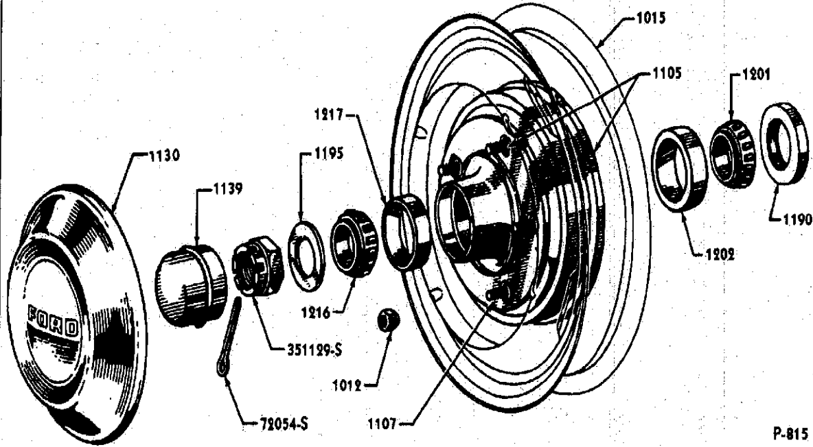
FRONT WHEEL, HUB, BEARINGS, ETC.
